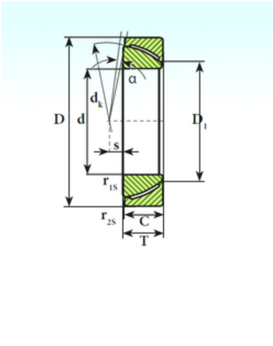
GAC 260 CP Bearing 2D drawings and 3D CAD models
