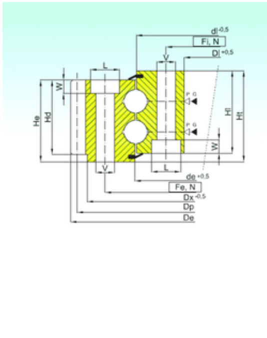
EB2.25.0980.400-1RPPN Bearing 2D drawings and 3D CAD models
